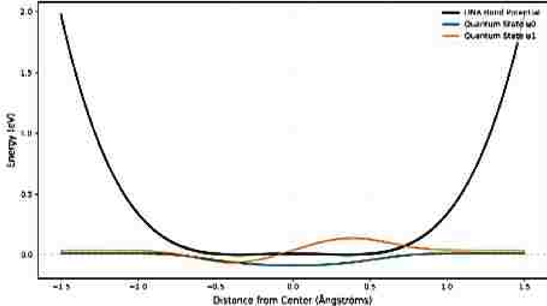
Proton Tunneling in Guanine-Cytosine Hydrogen Bond
